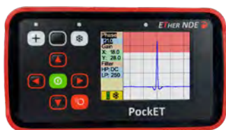
PockET Eddy Current Flaw Detector
