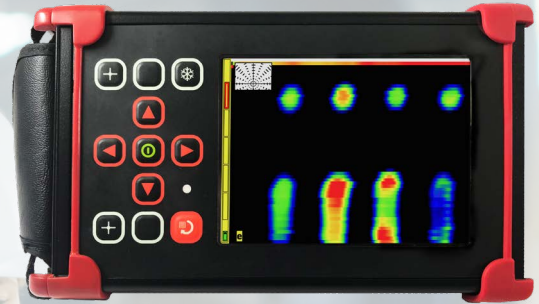
DUAL FREQUENCY HIGH PERFORMANCE EDDY CURRENT FLAW DETECTOR WITH C-SCAN CAPABILITY.
