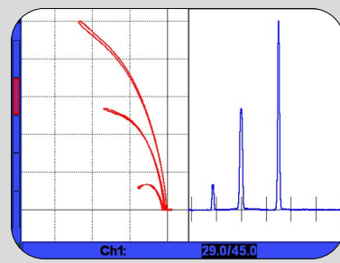
50/50 XY & Timebase
